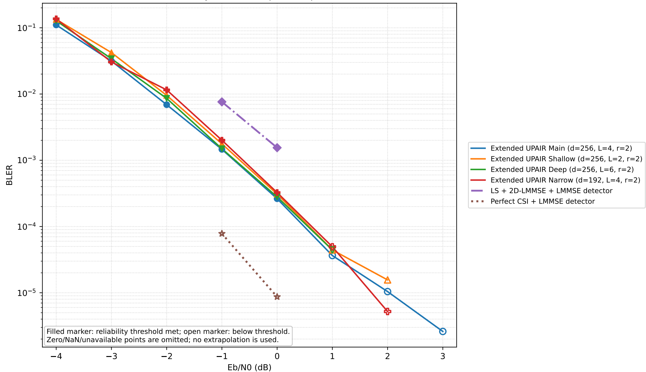
Extended UPAIR Variants and Available Benchmarks — BLER 3 active users — only evaluated, positive points are shown
